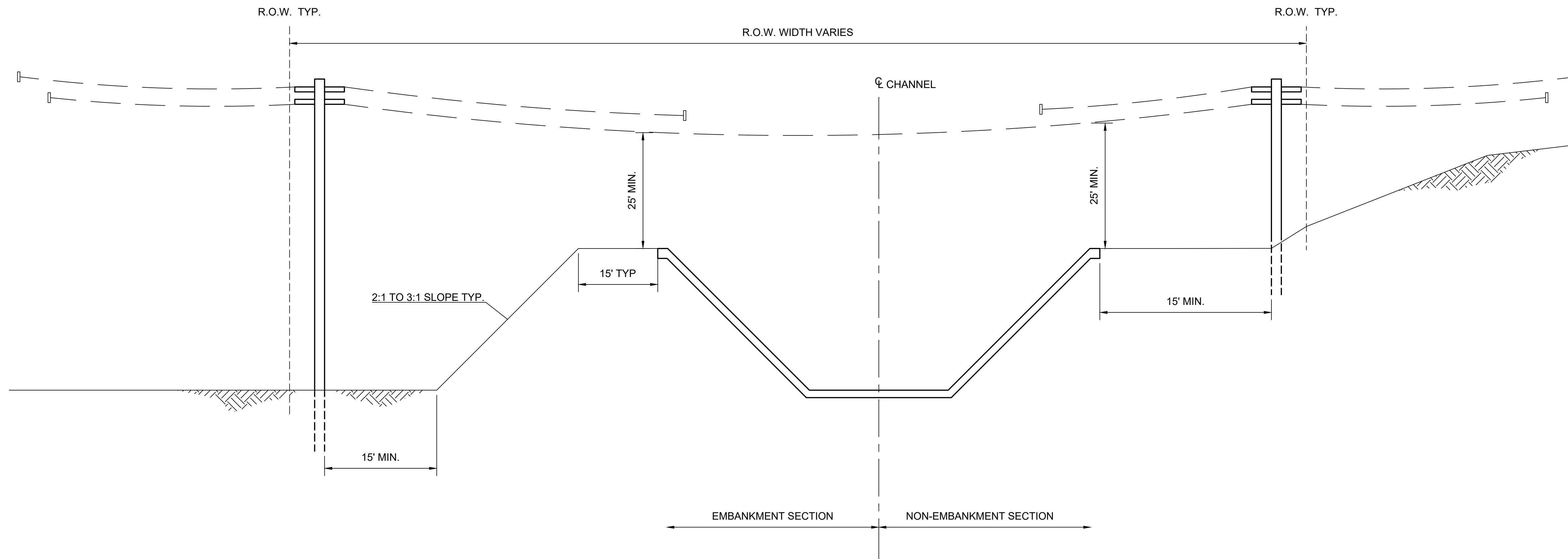
OVERHEAD UTILITY CROSSING NO SCALE
